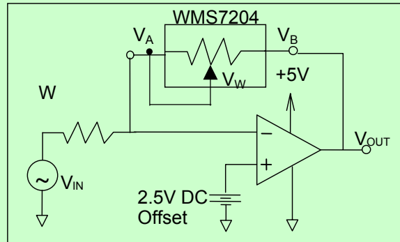
Capacitance test circuit
