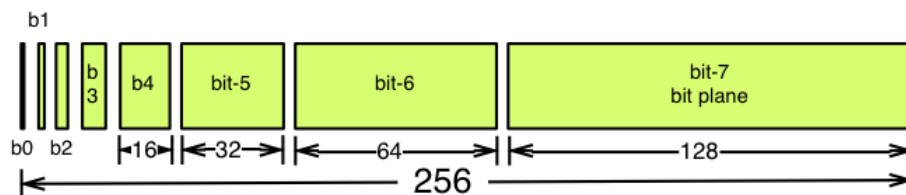
Figure 4-2. Relationship Between Bit Partition and Time
