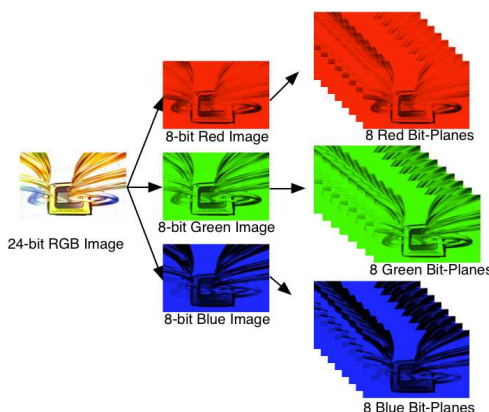
Figure 4-1. Relationship Between Bit Planes and 24-Bit RGB Images
