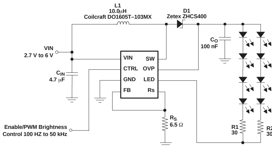
Figure 25. TPS61042 Powering 8 LEDs, Efficiency = 81%@ V_I = 3.6\text{ V}/18.6\text{ mA}
