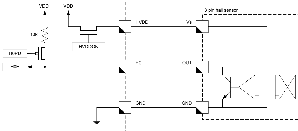
Figure 20. H0 Used as 3-Pin Hall-effect Sensor Input
