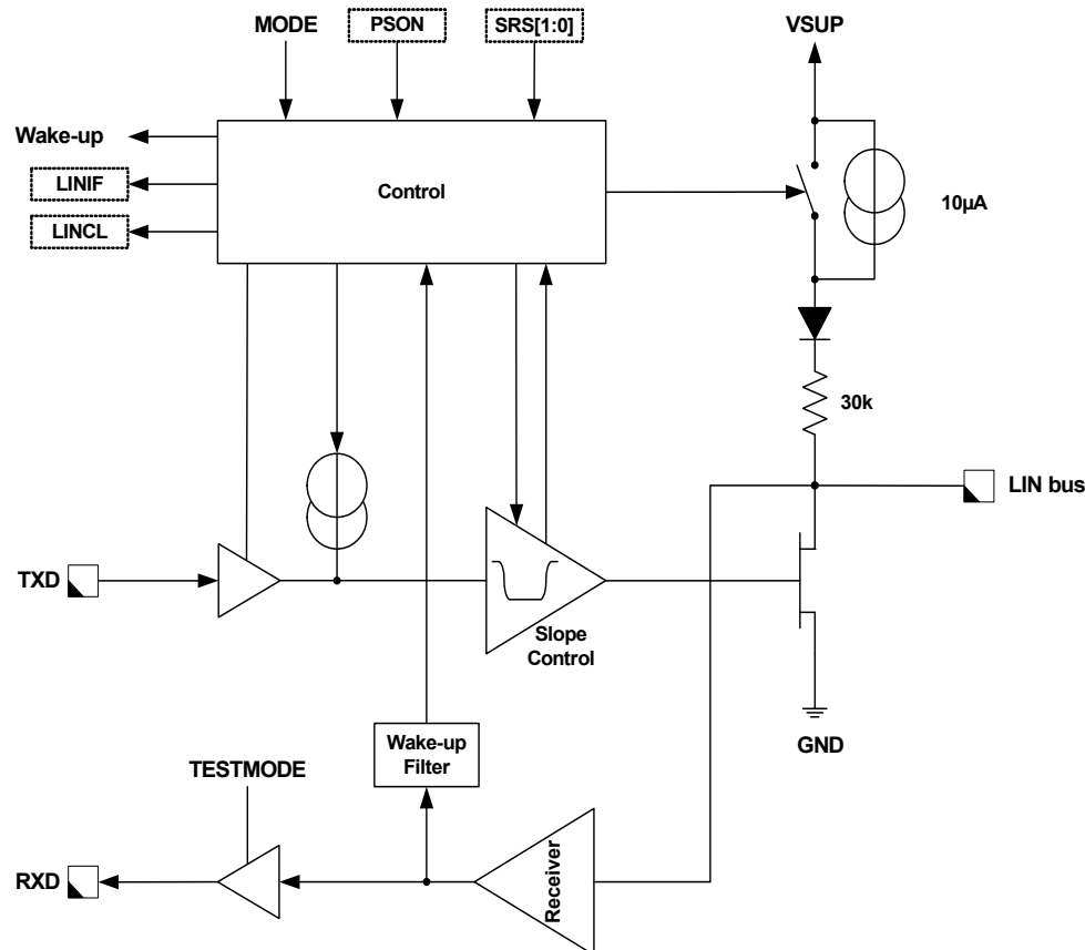
Figure 16. LIN Interface
