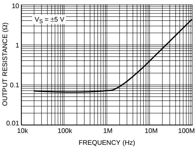
Figure 21. Closed-Loop Output Resistance vs. Frequency
