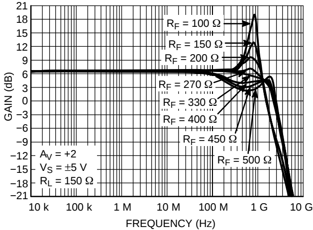
Figure 23. Frequency Response vs. R_F
