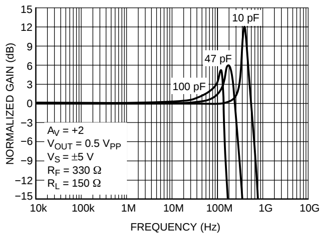
Figure 22. Frequency Response vs. Capacitive Load
