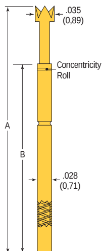
BGA & PGA Crown Head
