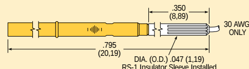
SR261-4 Quick Connect™
