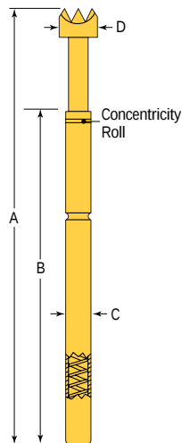
BGA & PGA Serrated Head
