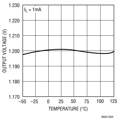
Output Voltage
