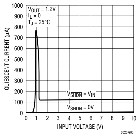
Quiescent Current
