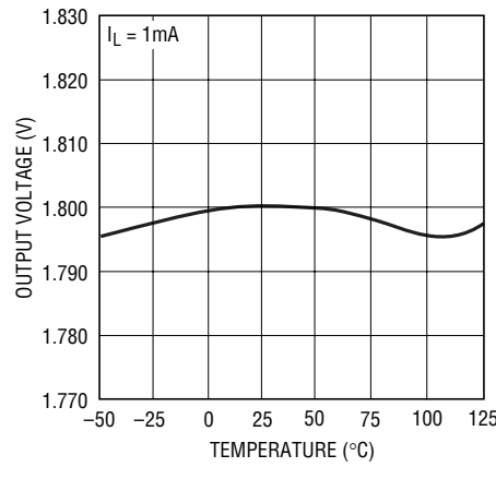
Output Voltage
