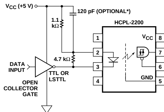
Figure 16. Series LED drive with open collector gate (4.7 kΩ resistor dhunts I OH from the LED).
