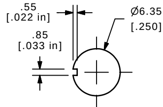
PANEL MOUNTING
