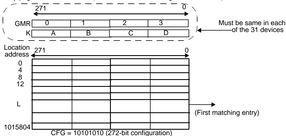
Figure 10-70. x272 Table with 31 Devices
