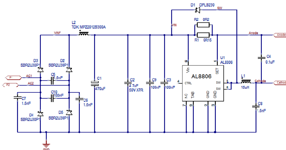
Figure 7 MR16 Schematic
