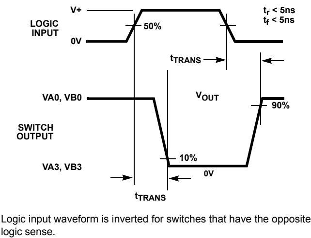
FIGURE 1C. ADDRESS tTRANS MEASUREMENT POINTS
