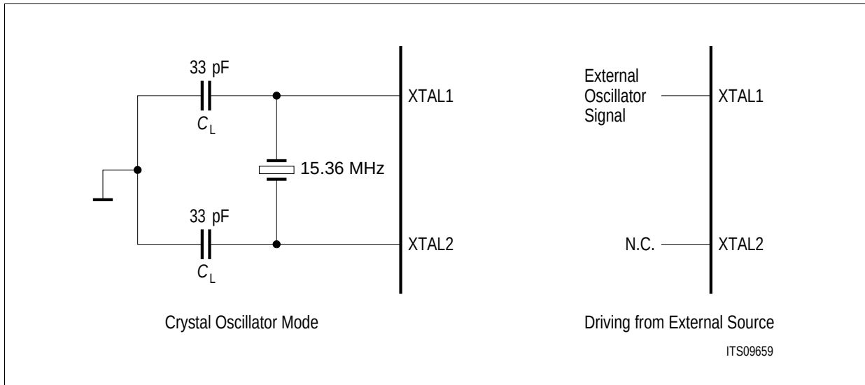
Figure 83 Oscillator Circuit
