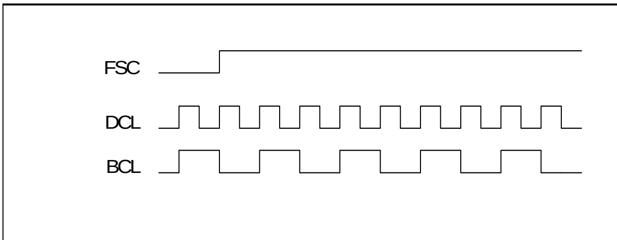
Figure 79 Clock waveforms
