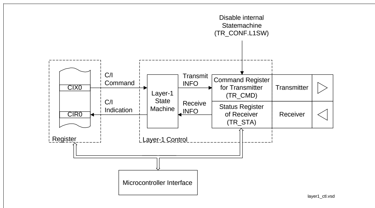
Figure 40 Layer-1 Control
