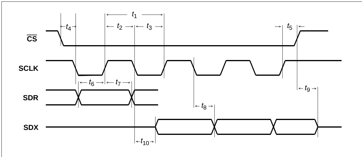
Figure 87 SCI Interface
