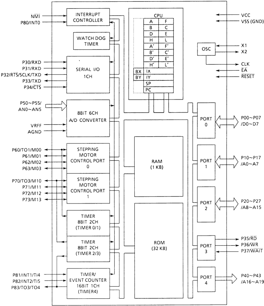
Figure 1. TMP90CM40 Block Diagram
