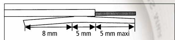
"PULL-UP" VERSION
