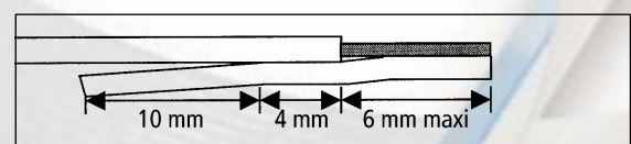
"EASY-TO-INSERT" VERSION
