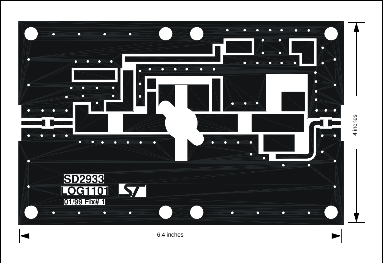
Figure 12. 30 MHz Test Circuit Photomaster
