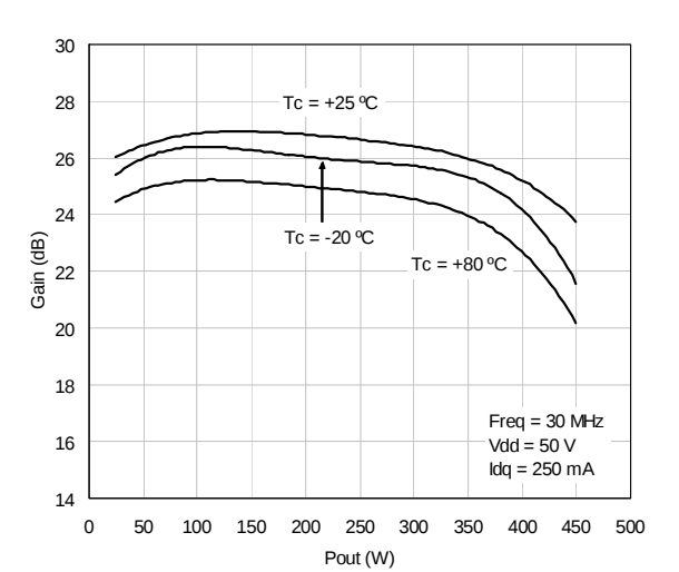
Figure 8. Power Gain Vs Pout & Case Temp.
