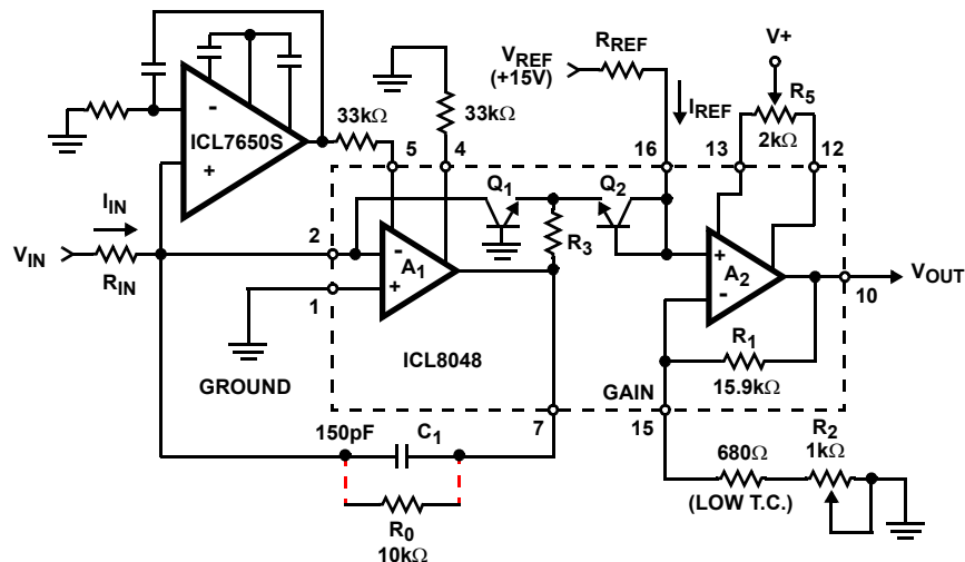
FIGURE 6. ICL8048 OFFSET NULLED BY ICL7650S
