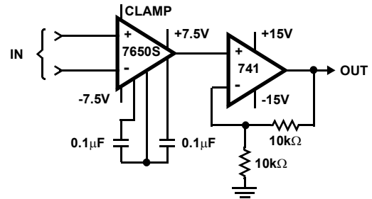
FIGURE 4. USING 741 TO BOOST OUTPUT DRIVE CAPACITY
