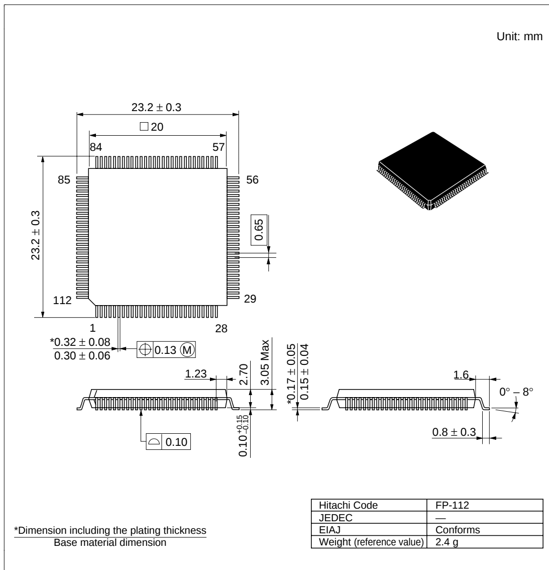
Figure F.1 Package Dimensions (FP-112)
