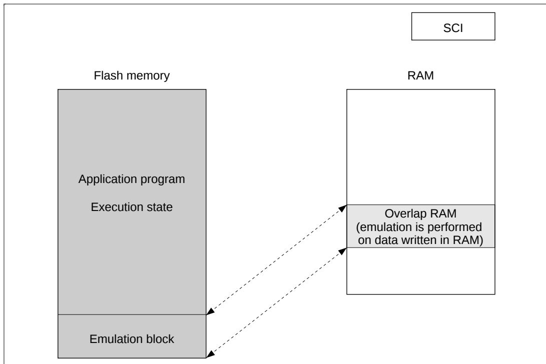
Figure 18.5 Emulation
