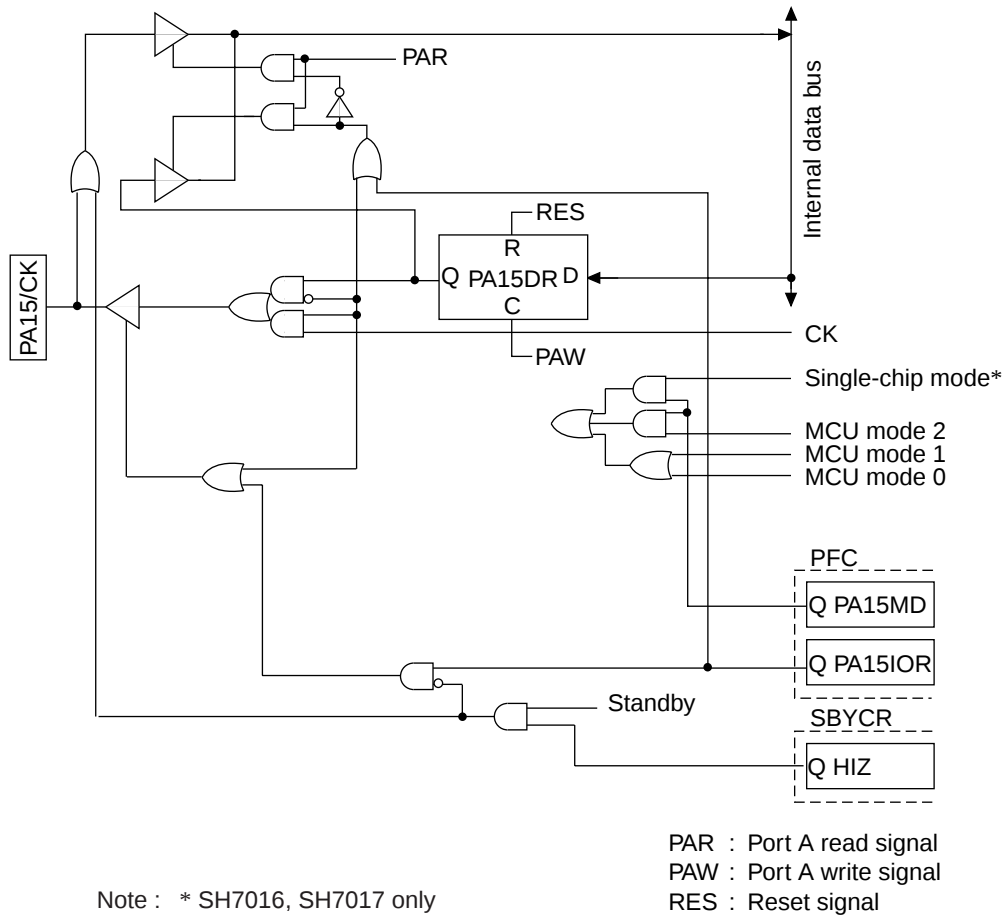
Figure B.8 PA15/CK Block Diagram
