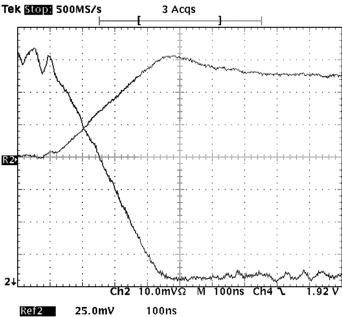
Figure 2(b). Output Transient Response of Figure 1 Circuit, I_{OUT} from 14A to 0A (Reference 2 = V_{OUT} , Channel 2 = I_{OUT} ).
