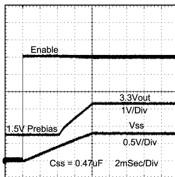
Figure 46. Prebiased Start-Up
