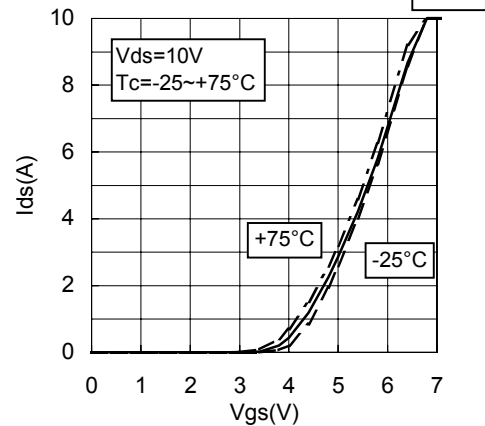
Vgs-Ids CHARACTERISTICS 2
