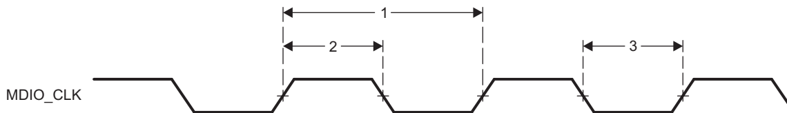
Figure 7-4. MDIO_CLK Timing
