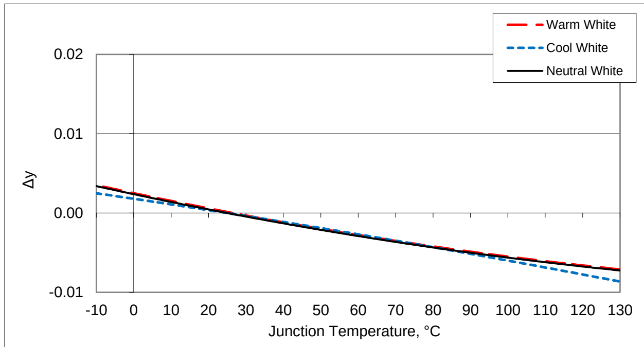
Figure 4: Typical ccy Shift vs. Junction Temperature
