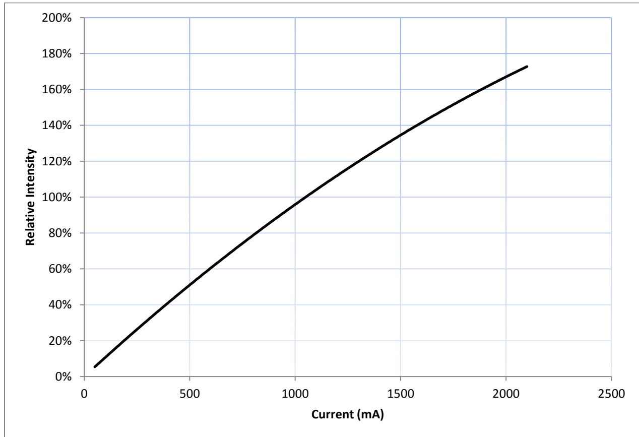
Figure 2: Typical Flux vs. Current, T_j = 25^{\circ}\text{C}
