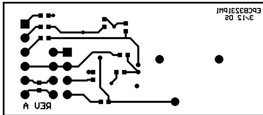
Figure 6. DS3231MPMB1 Peripheral Module PCB Layout—Solder Side
