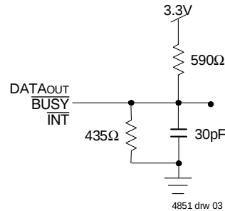
Figure 1. AC Output Load
