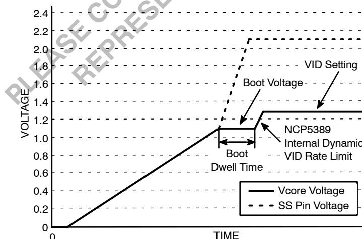
Figure 7. Typical VR11 Soft-Start Sequence to Vcore = 1.3 V
