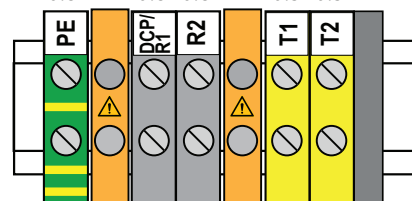
Terminals FSC Braking Resistor
