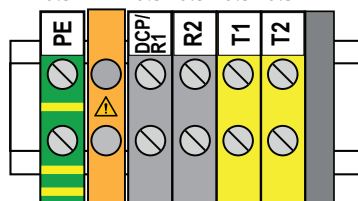
Terminals FSB Braking Resistor
