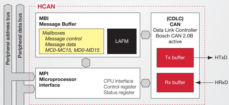
HCAN Block Diagram
