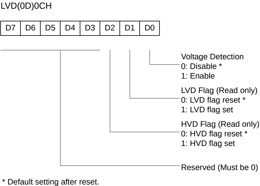
Figure 43. Voltage Detection Register
