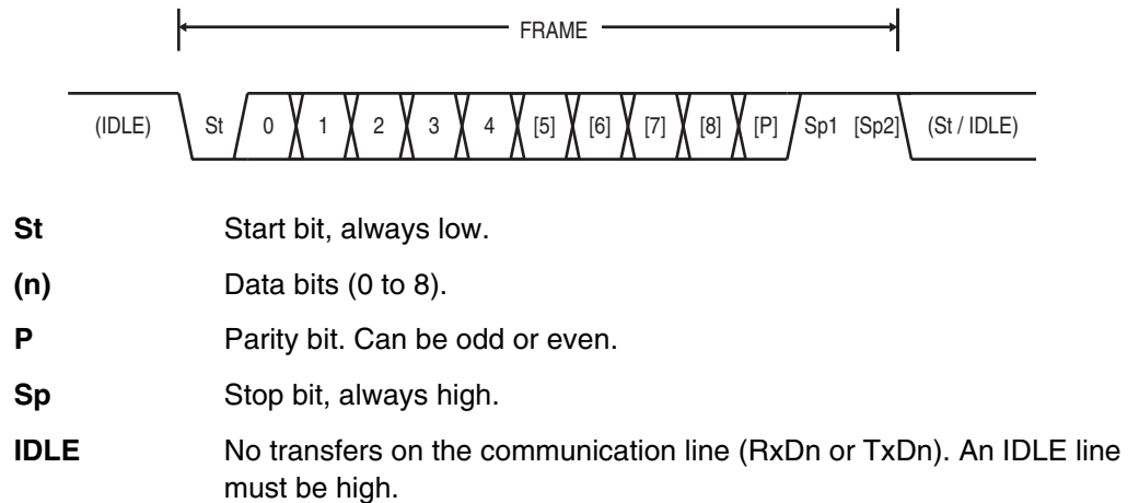
Figure 4-72. Frame Formats
