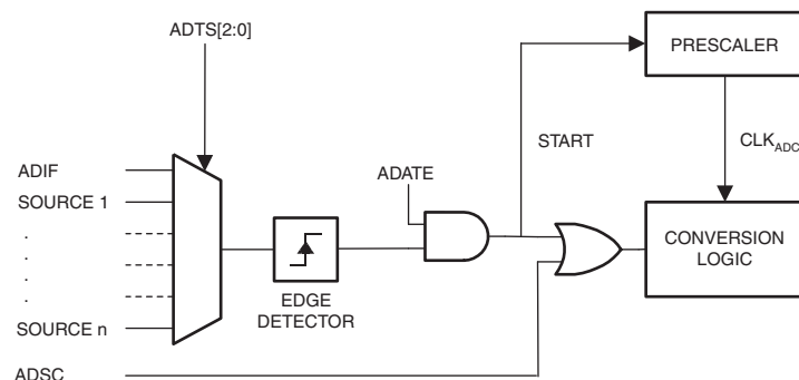
Figure 4-101. ADC Auto Trigger Logic
