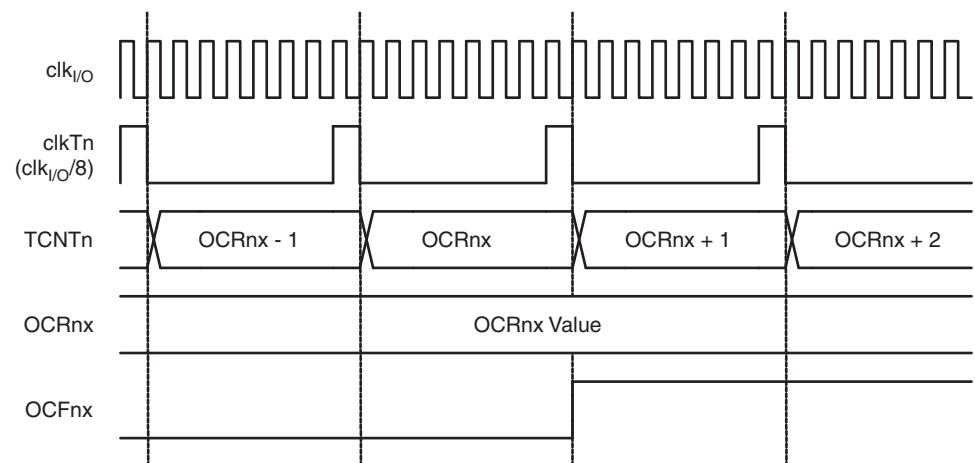
Figure 4-50. Timer/Counter Timing Diagram, Setting of OCF1x, with Prescaler ( f_{\text{clk}_{I/O}}/8 )
