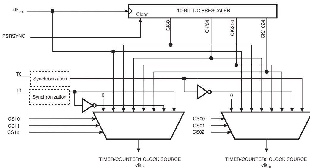
Figure 4-39. Prescaler for Timer/Counter0 and Timer/Counter1 (1)
