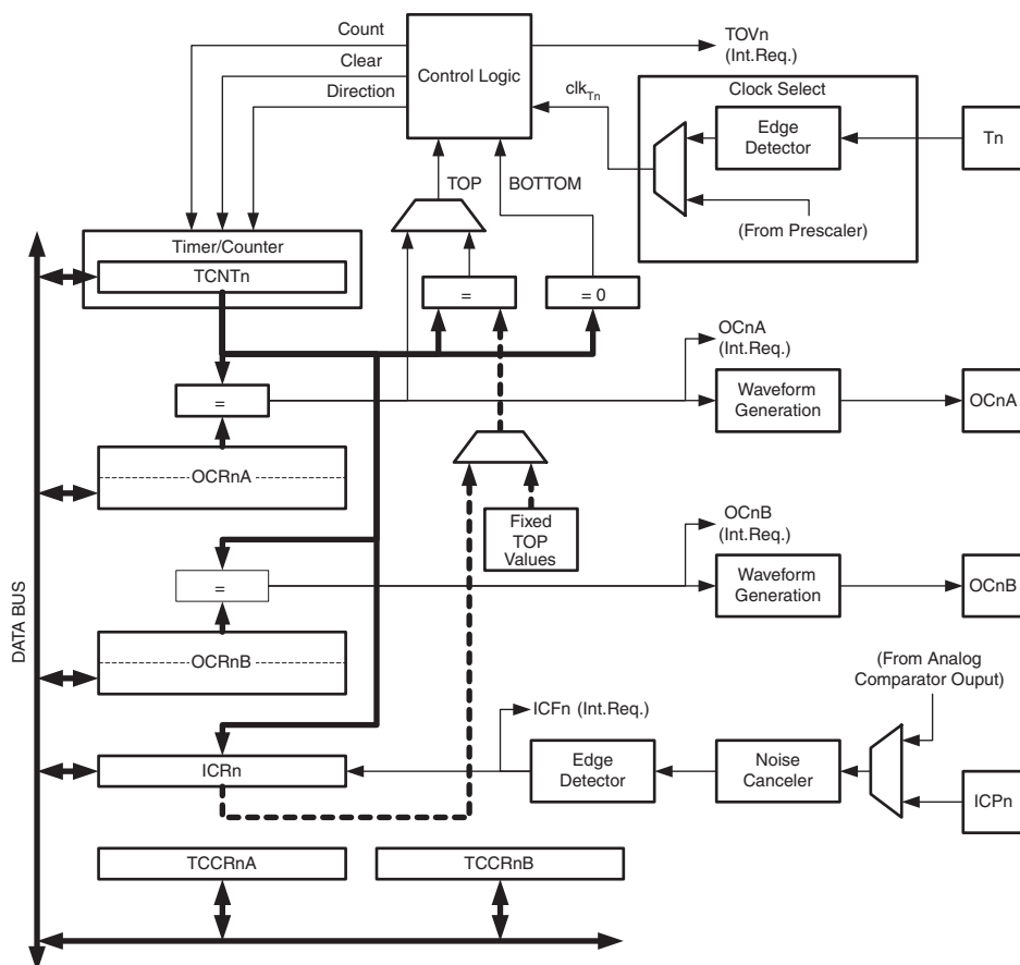
Figure 4-40. 16-bit Timer/Counter Block Diagram (1)
