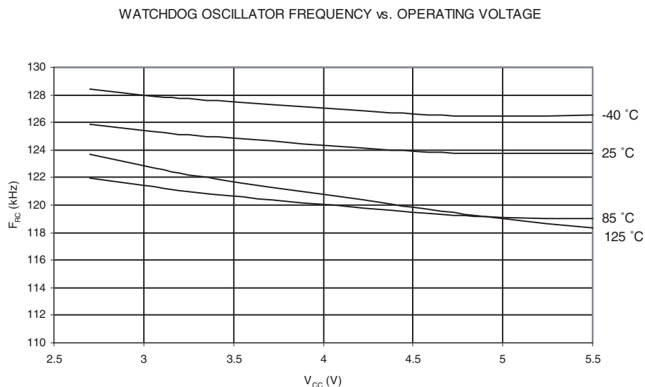
Figure 5-22. Watchdog Oscillator Frequency vs. V_{CC}
