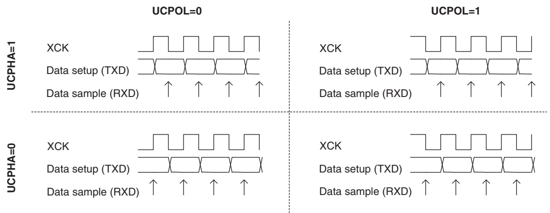
Figure 4-76. UCPHAN and UCPOLn Data Transfer Timing Diagrams
