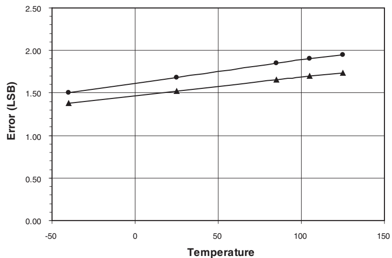
Figure 5-31. Analog to Digital Converter OFFSET versus V_{CC}
