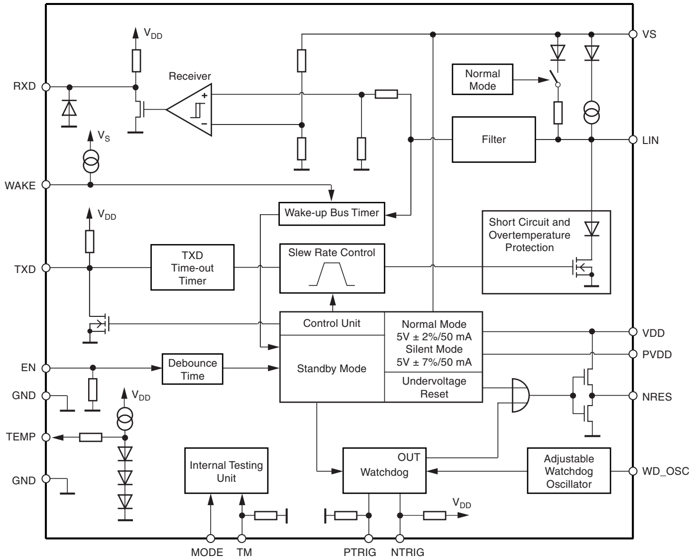
Figure 3-1. Block Diagram
