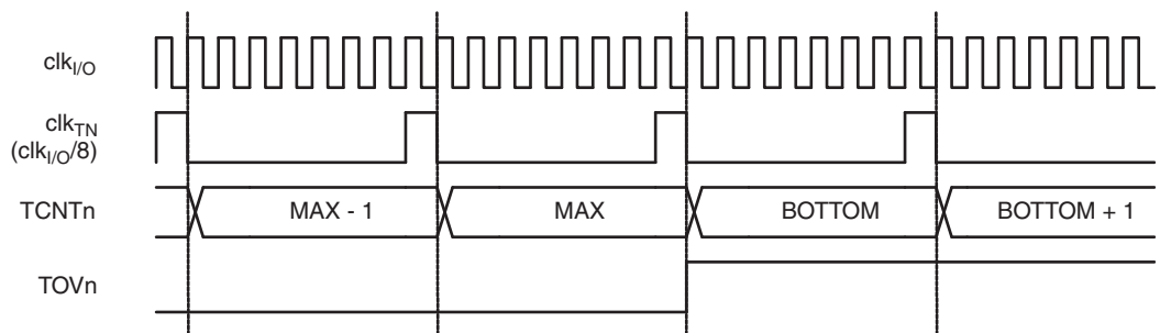
Figure 4-35. Timer/Counter Timing Diagram, with Prescaler ( f_{\text{clk\_I/O}}/8 )
