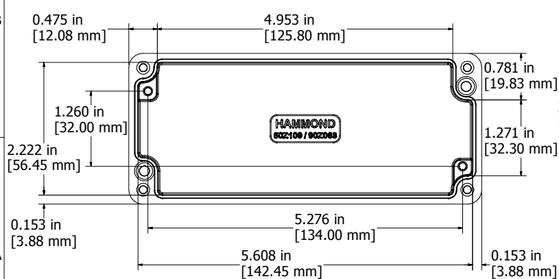
Top View Looking Inside Box
