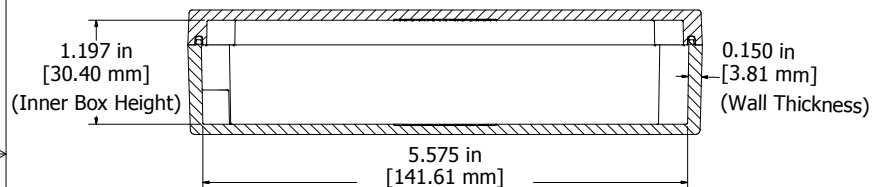
SECTION B-B Side View of Assembly
