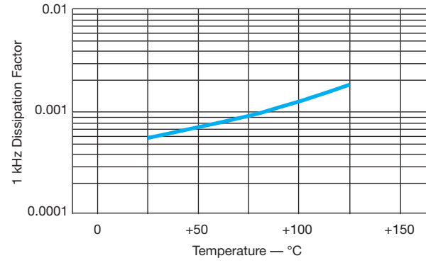
Dissipation Factor vs. Temperature Axial
