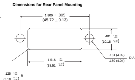
Dimensions for Rear Panel Mounting
