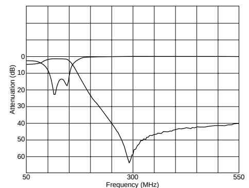
Frequency Characteristics
