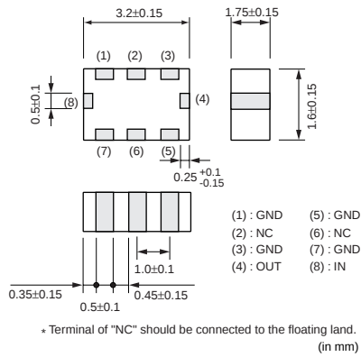
LFL31 Series
