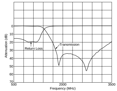
Frequency Characteristics
