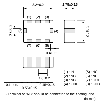
LFL32 Series
