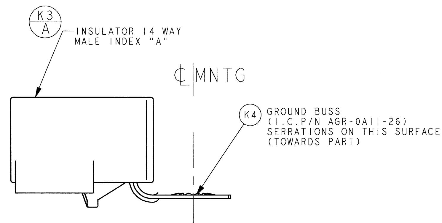
ASSY GROUND BUSS 180° P/N 04688938
