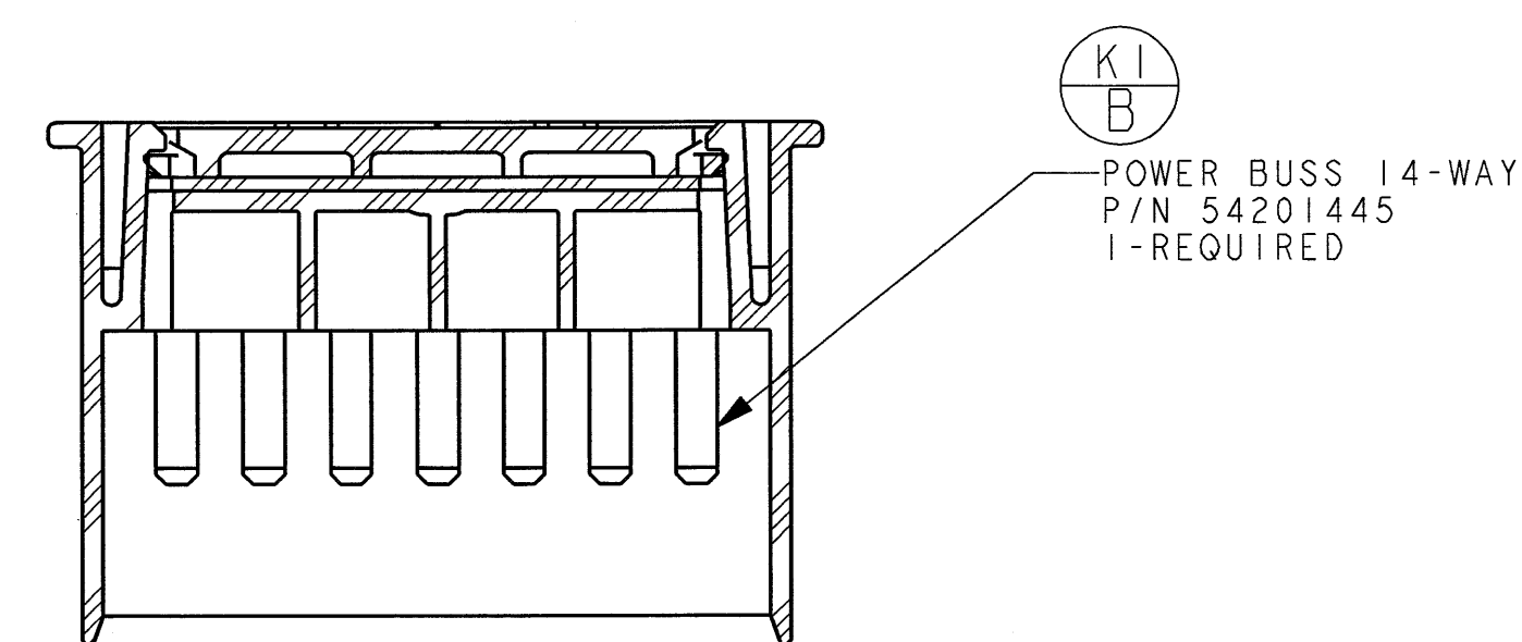
SECTION B-B ASSY POWER BUSS P/N 54201465
