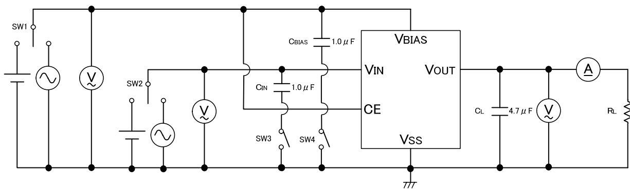
Circuit ③
