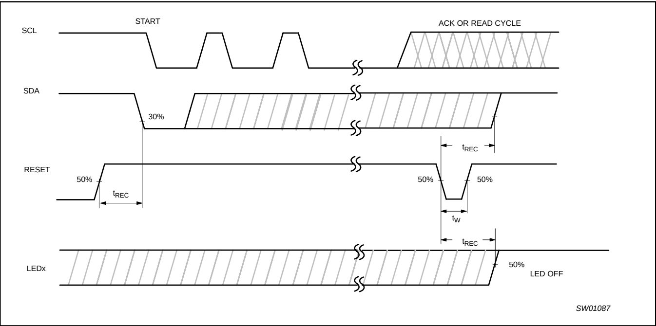
Figure 18. Definition of \overline{\text{RESET}} timing
