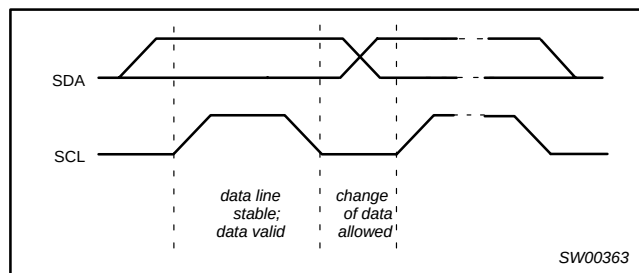
Figure 6. Bit transfer
