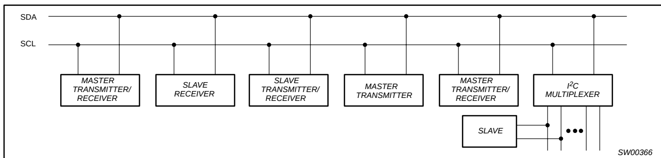
Figure 8. System configuration
