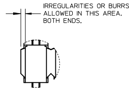
DETAIL Z SCALE 5:1
