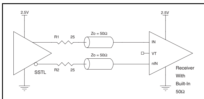
Figure 3E. HiPerClockS IN/nIN Input with Built-In 50 \Omega Driven by an SSTL Driver
