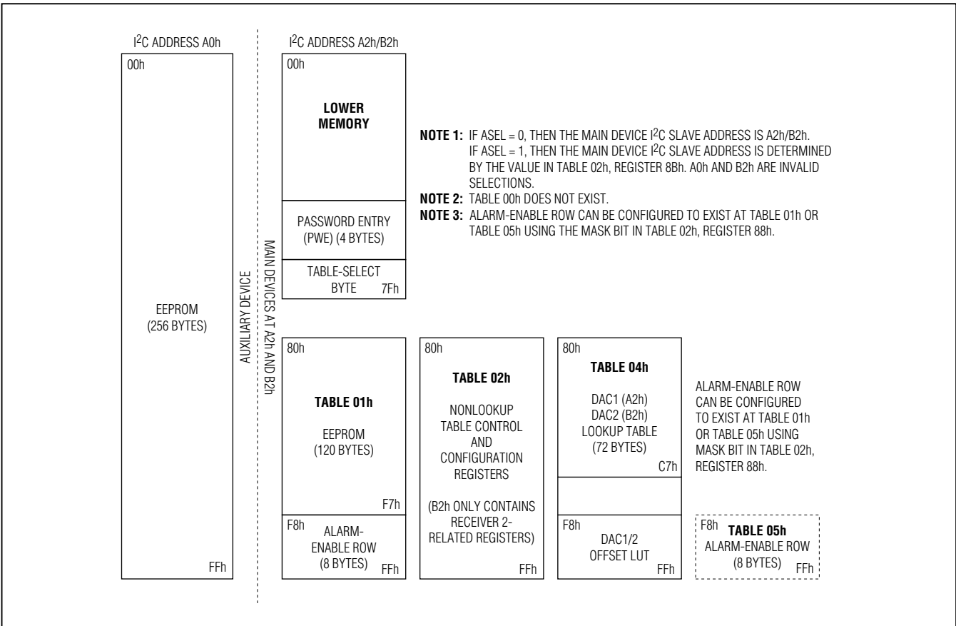
Figure 14. Memory Map
