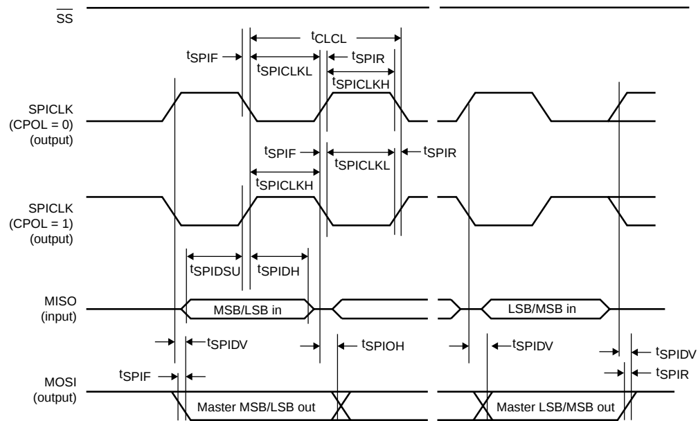
Fig 16. SPI master timing (CPHA = 1).
