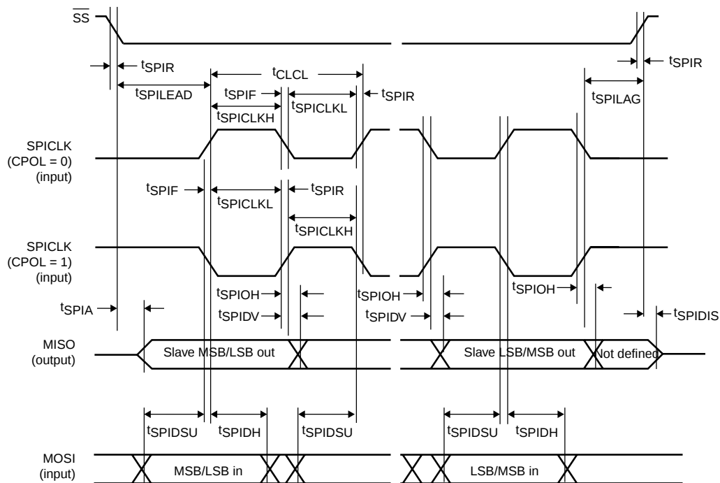
Fig 17. SPI slave timing (CPHA = 0).
