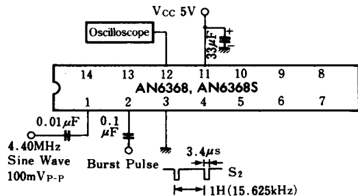
Test Circuit 2 ( S_2 , G_{V-12} )
