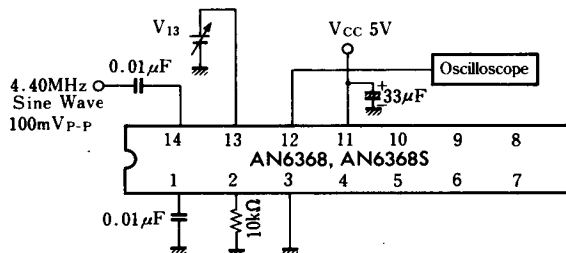
Test Circuit 4 ( V_{H-9} , V_{H-8} , I_{S-7} )
