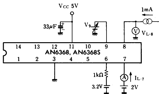
Test Circuit 5 ( V_{L-9} , V_{L-8} , I_{L-7} )
