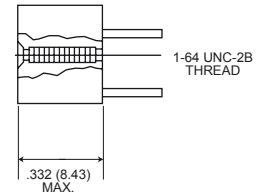
Plug
