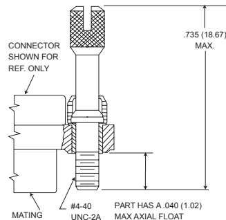
Jackscrew - (K) Standard
