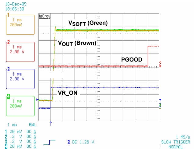
FIGURE 14. SOFT-START WAVEFORM SHOWING PGOOD
