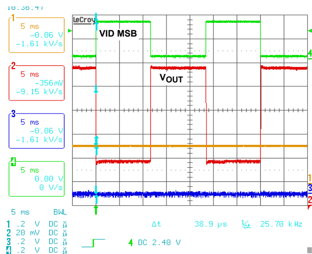
FIGURE 23. VID MSB BIT CHANGE FROM 1.4375V TO 0.65V SHOWING 9mV/μs SLEW RATE, DPRSLPVR = 0, DPRSTP# = 1
