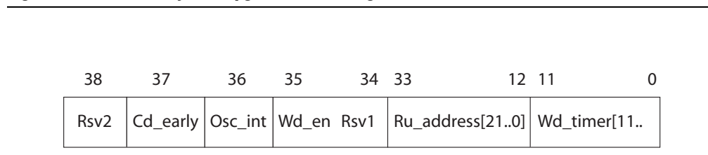
Figure 9-36. Remote System Upgrade Control Register
