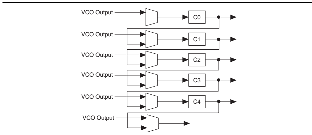
Figure 5-12. Counter Cascading
