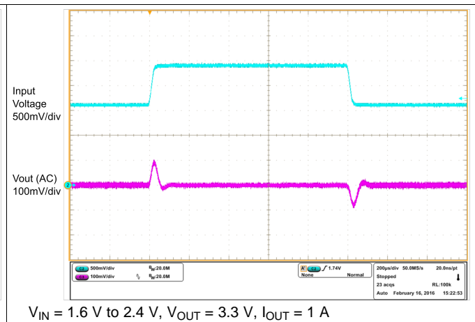
Figure 17. Line Transient
