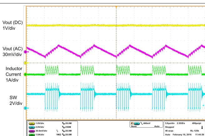
Figure 13. Switching Waveform at Light Load
