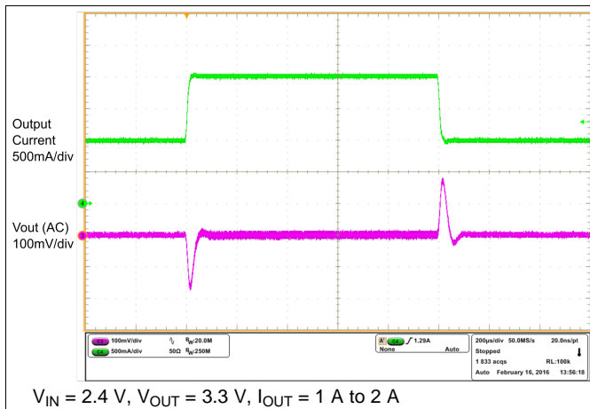
Figure 16. Load Transient
