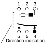
2-coil latching
