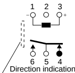
1-coil latching
