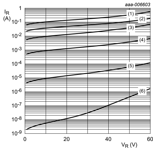
pulsed condition (1) T_j = 175^\circ\text{C} (2) T_j = 150^\circ\text{C} (3) T_j = 125^\circ\text{C} (4) T_j = 85^\circ\text{C} (5) T_j = 25^\circ\text{C} (6) T_j = -40^\circ\text{C}
