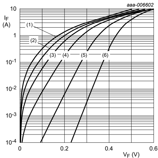
pulsed condition (1) T_j = 175^\circ\text{C} (2) T_j = 150^\circ\text{C} (3) T_j = 125^\circ\text{C} (4) T_j = 85^\circ\text{C} (5) T_j = 25^\circ\text{C} (6) T_j = -40^\circ\text{C}
