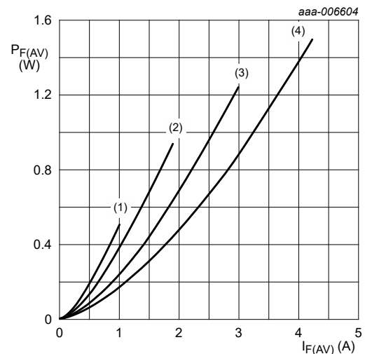
T_j = 175^\circ\text{C} (1) \delta = 0.1 (2) \delta = 0.2 (3) \delta = 0.5 (4) \delta = 1
