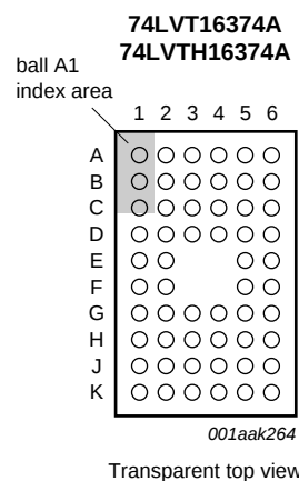
Fig 5. Pin configuration for SOT702-1 (VFBGA56)
