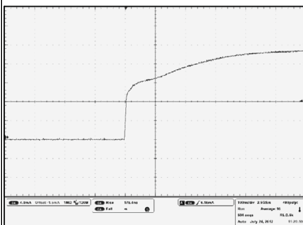
Figure 19. Output T_{ON} (current rise time) CFG - 12 = CFG - 11 = 1
